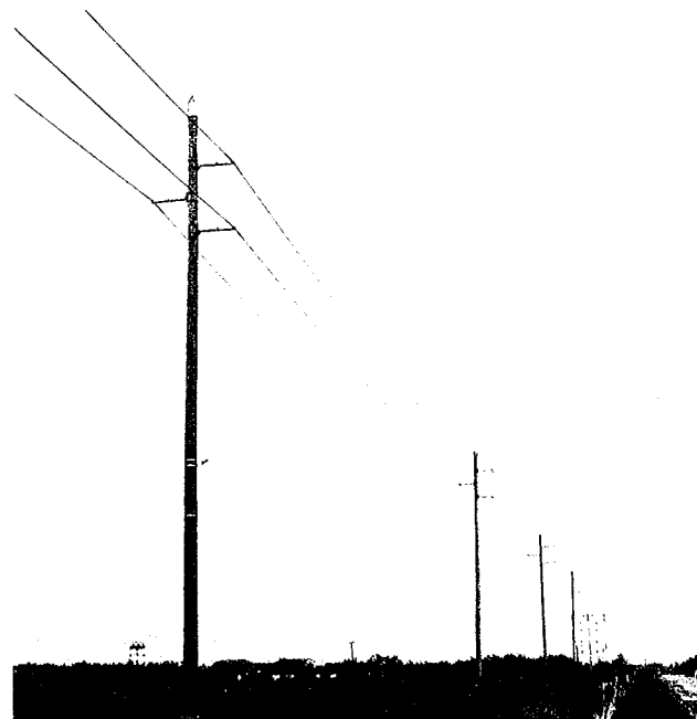
Lapp Resistance Graded (RG) Horizontal Line Posts on wood poles on this 115 kv line in the Gulf Coast area were used to combat severe salt fog contamination and reduce high cost of washing insulators.
