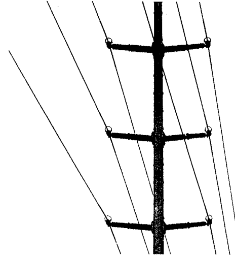
Double circuit concrete pole 138 kv transmission. Horizontally mounted RG Line Posts provide neat appearance and contamination control in residential neighborhoods.
