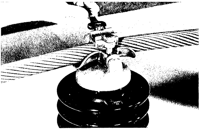
Recommended torque for tightening keeper capscrews on Clamp Top clamps is 25 foot pounds.
