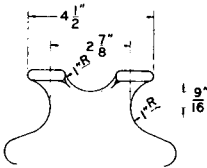
"F" Neck 25, 35, 45 kv
