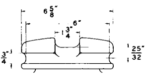
"N" Neck 55, 66, 88 kv
