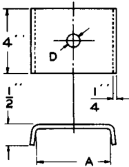
Fig. 1 Crossarm Saddle
