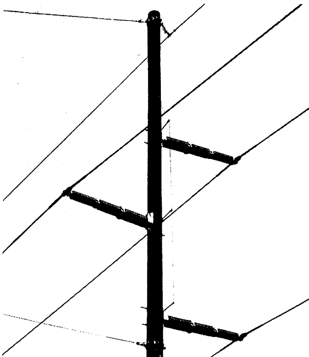
Lapp 161 kv Horizontal Line Post for wood pole mounting.
