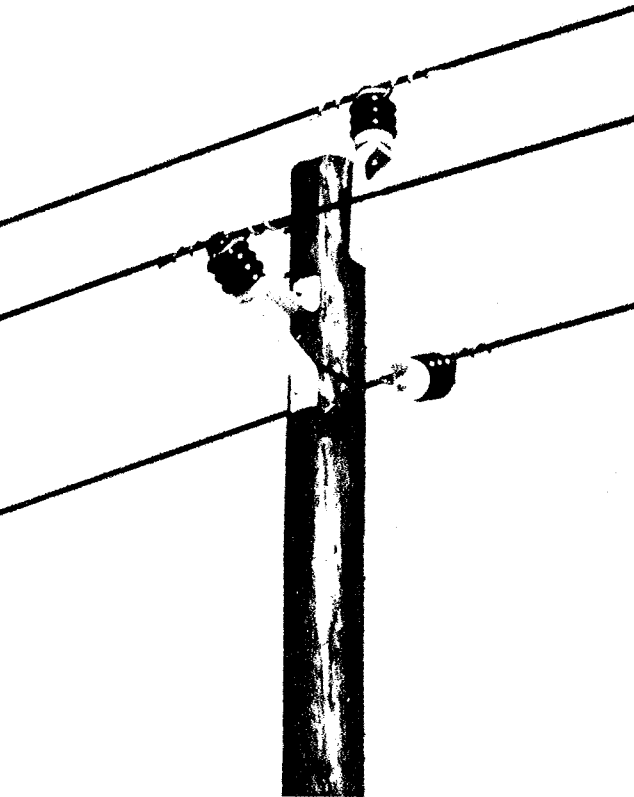
Stud mounted Distribution Posts on Lapp offset pole mounting brackets provide necessary conductor clearances on long spans. Offset pole mounting brackets are shown on page 6.
