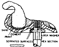
Mounting Base Detail
