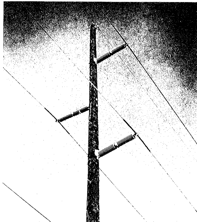
The trim, low voltage appearance of this 115 kv shielded delta configuration on wood poles is one of the reasons why armless construction on Lapp Horizontal Line Posts has proved so popular for urban and suburban transmission construction.
