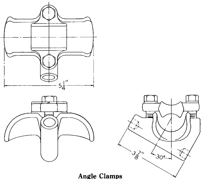
Angle Clamps
